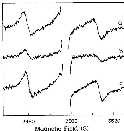
Fig. 2. EPR spectra of ether-linked PC liposomes loaded with tempocholine and suspended in ascorbate-containing buffer. The central parts of the spectra have been deleted to avoid overlap of the ascorbyl radical lines. (a) No additions; (b) after addition of 0.8 mg/ml ammodytin L; (c) after addition of 0.8 mg/ml Naja PLA 2 plus 1 mM Ca 2+ .
