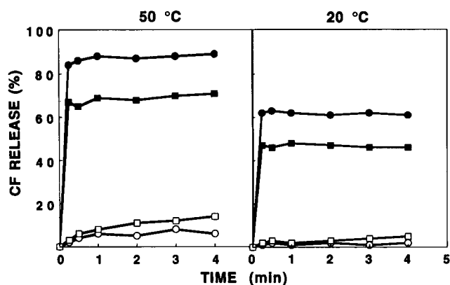
Fig. 1. Time-course of CF leakage induced by 1 \mu M (●) or 0.5 \mu M of ammodytin L (■), 1 \mu M Naja PLA 2 (□) or in the absence of proteins (○) from liposomes of O-PC/O-PA (9:1, mol/mol) in 20 mM Tris-HCl (pH 7.4). At time zero, proteins were added to the liposome suspension; the fluorescence of samples was monitored at two different temperatures: 50°C (left panel) and 20°C (right panel).
